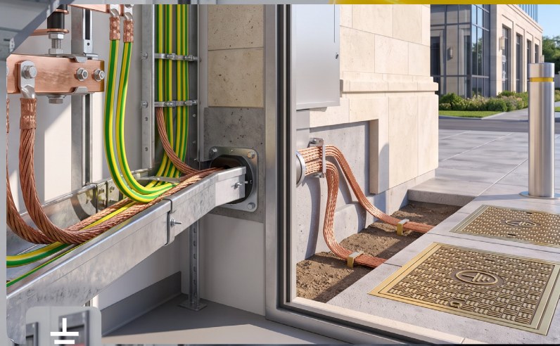
● Earthing Ground System
